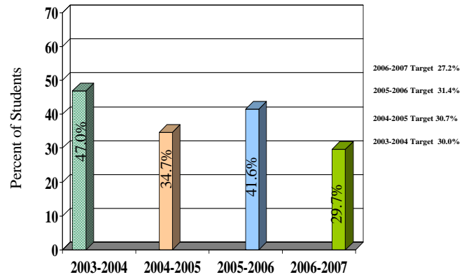
AMAO 2 Results
