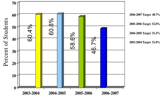
AMAO 1 Results
